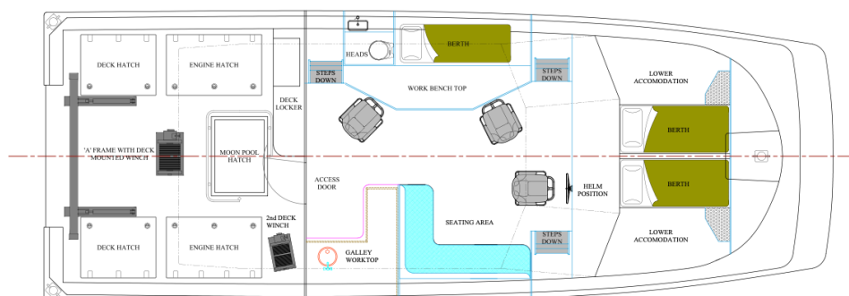
TOP VIEW - DECK LEVEL
