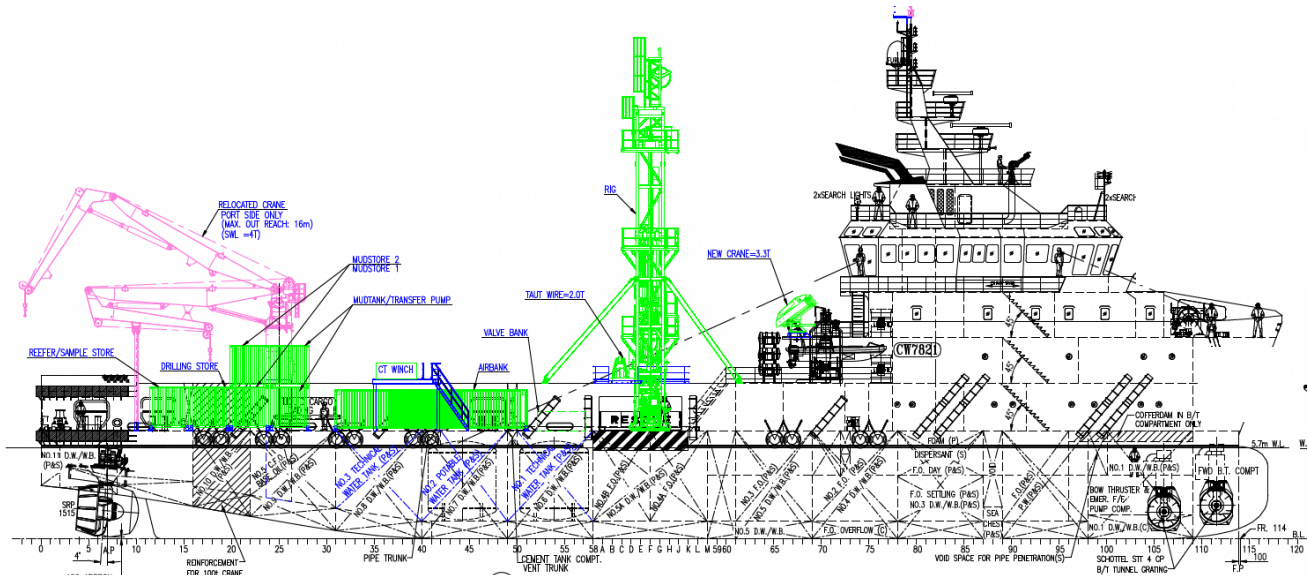
SIDE VIEW - PORT SIDE
