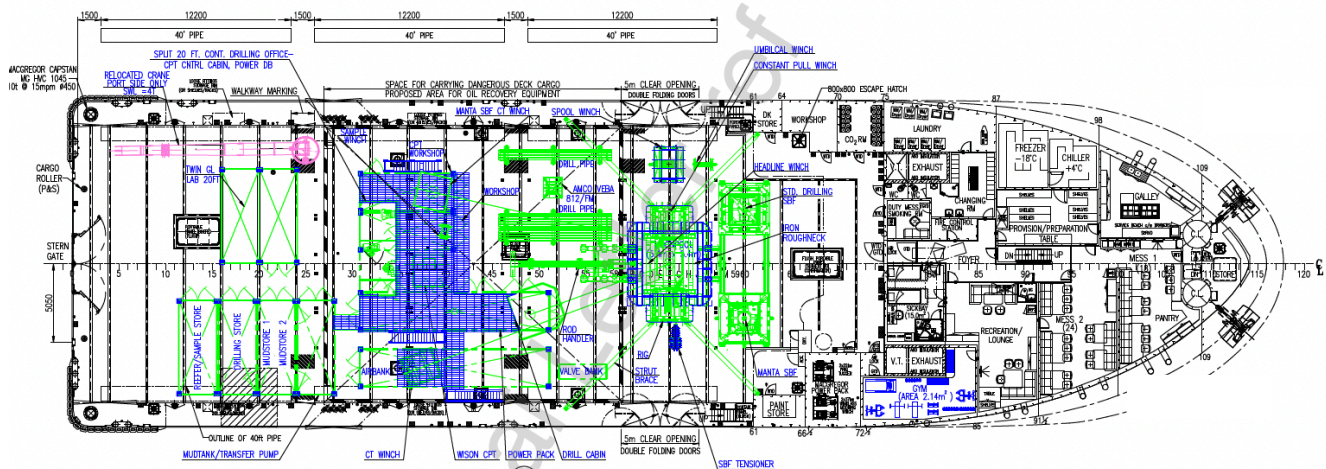
TOP VIEW - DECK LEVEL
