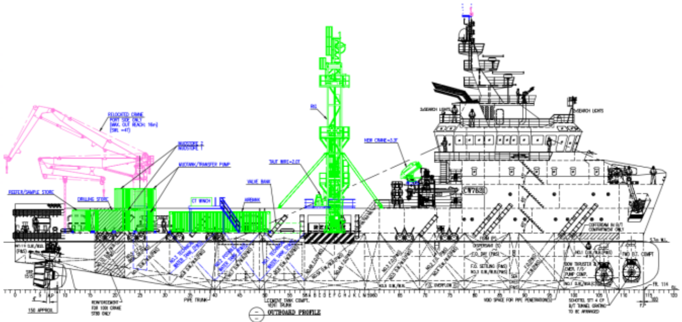
SIDE VIEW - PORT SIDE
